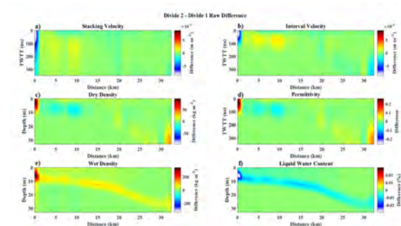
Fig. 1. The difference in (a) stacking velocity, (b) interval velocity, (c) dry density, (d) permittivity, (e) wet density and (f) LWC from repeat 500 MHz MO GPR surveys show the spatial variability of these properties after one week.
