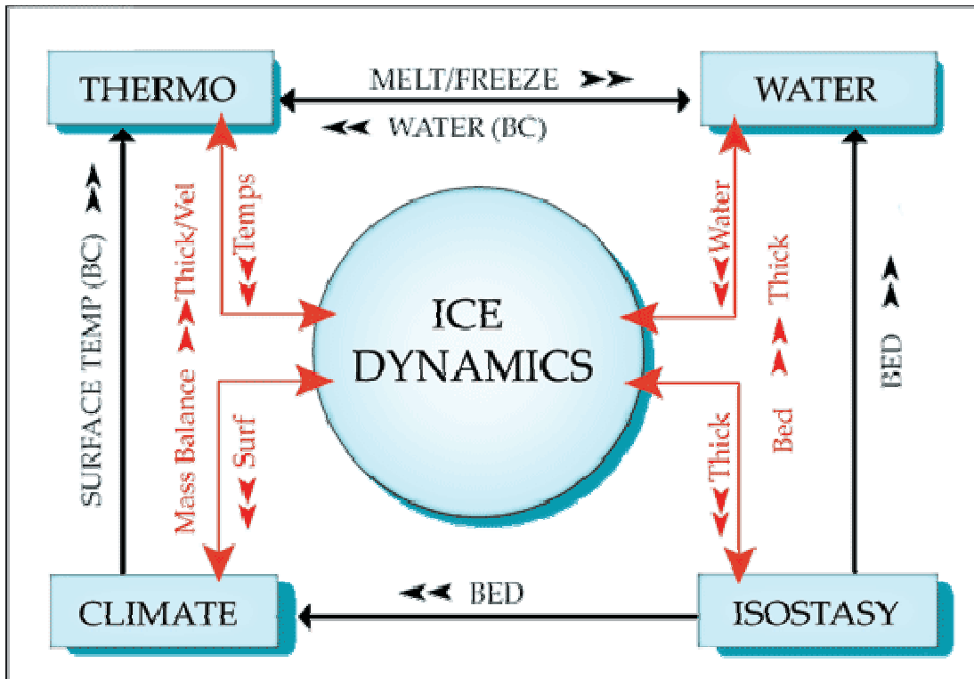
Graphic depicting the complex interaction of all of the factors mentioned above that go into the ice sheet model.
