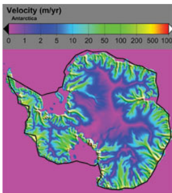
Antarctic reconstruction of present-day ice sheet showing velocities, basal water, and basal temperature. The bed at the melting point produces water which lubricates the ice streams.
